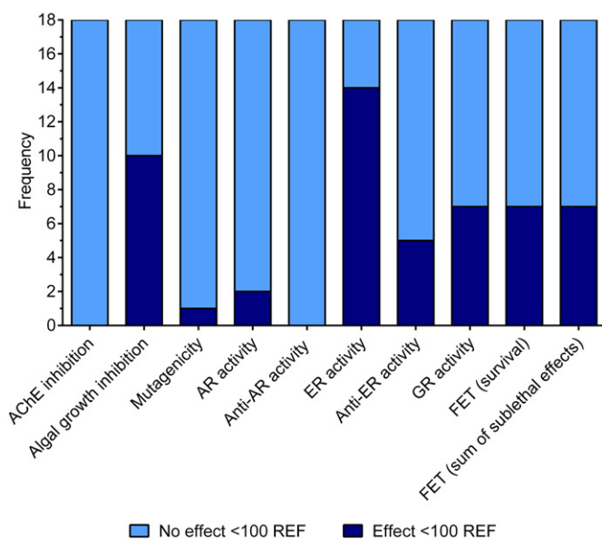
Fig. 5. Occurrence of responses in bioassays to 18 LVSP50 samples collected during the European demonstration program; most samples were tested in most bioassays up to a REF of 100, except AChE (up to REF 500); REF: relative enrichment factor; AChE: acetylcholinesterase enzymatic inhibition, AR: androgenic mediated activity, ER: estrogenic mediated activity, GR: glucocorticoid receptor mediated signalling, FET: zebrafish embryo test (Tousova et al., unpublished data).
