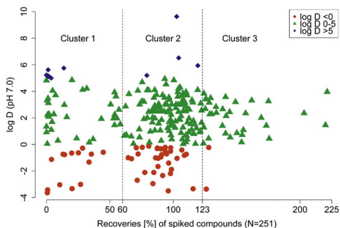
Fig. 4. Scatterplot of the total recoveries (in %) of compounds ( N = 251 ) spiked in a pristine water sample of Wormsgraben (Harz Mountains, Germany) and extracted with the LVSP50 device versus the water-ocanol partition coefficient at pH 7.0 corrected for the speciation ( \log D ); the dashed lines express the limits of the clusters derived from k -means cluster analysis ( k = 3 ); the plot shows only the data for HR-X.
